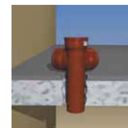
Insert the new branch long tail into the slab
