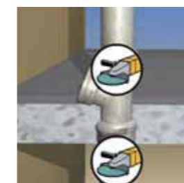
Cut the existing branch just above the slab
