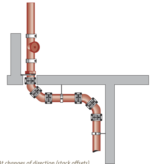
At changes of direction (stack offsets).
